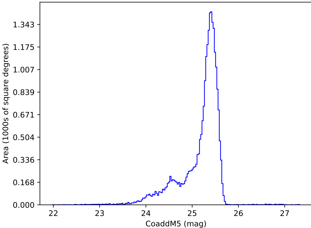
roll_uniform_early_half_mjdp67_v3.4_10yrs u: CoaddM5
