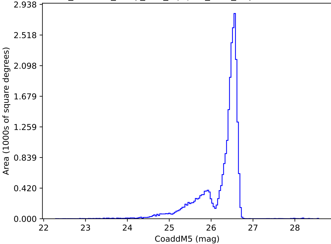
roll_uniform_early_half_mjdp67_v3.4_10yrs i: CoaddM5
