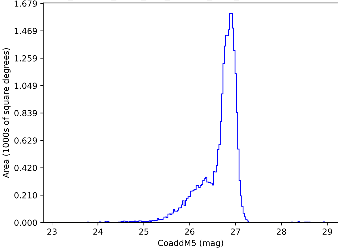
roll_uniform_early_half_mjdp67_v3.4_10yrs g: CoaddM5
