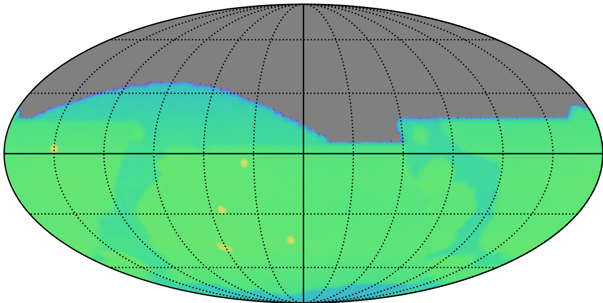
roll_uniform_early_half_mjdp67_v3.4_10yrs : CoaddM5
