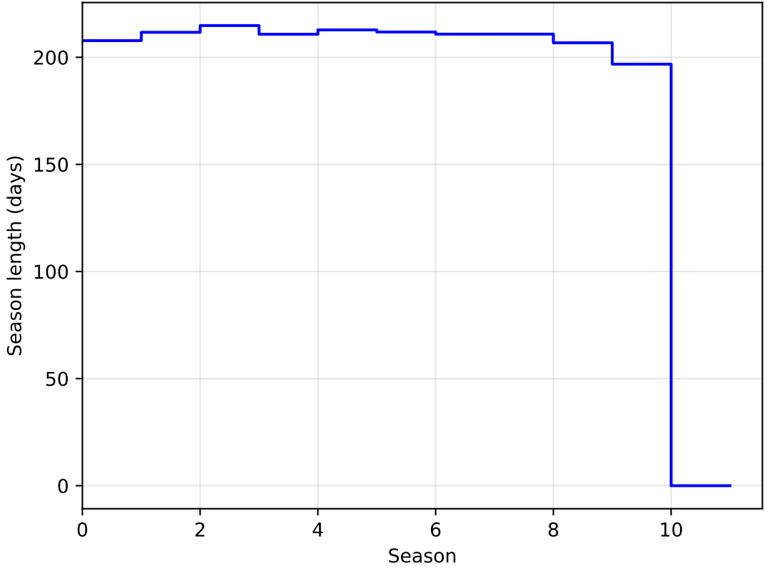
roll_uniform_early_half_mjdp67_v3.4_10yrs DD:EDFS all bands: SeasonLength
