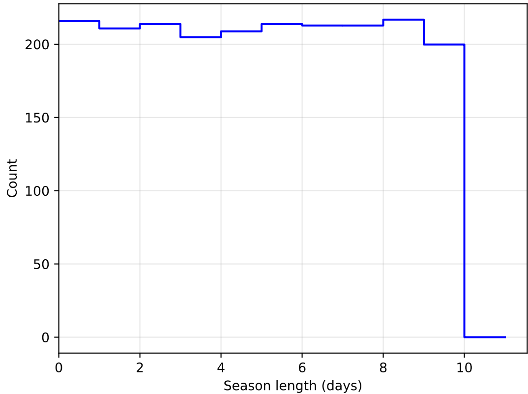
roll_uniform_early_half_mjdp67_v3.4_10yrs DD:ECDFS all bands: SeasonLength
