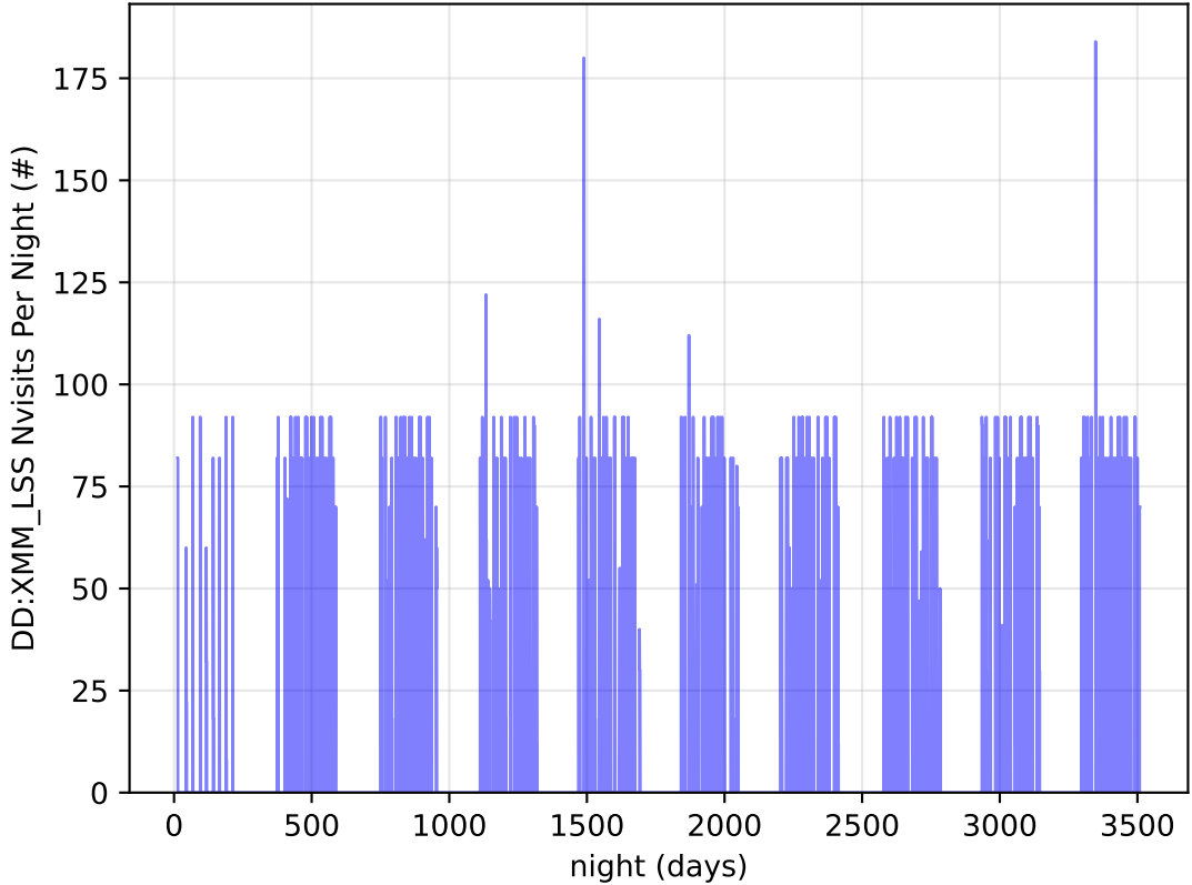
roll_uniform_early_half_mjdp67_v3.4_10yrs all bands: DD:XMM_LSS Nvisits Per Night
