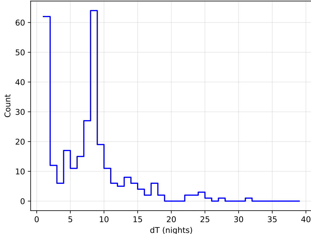
roll_uniform_early_half_mjdp67_v3.4_10yrs all bands: DD:XMM_LSS Delta Nights Histogram
