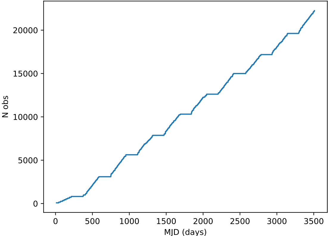
roll_uniform_early_half_mjdp67_v3.4_10yrs all bands: DD:XMM_LSS Cumulative NVisits
