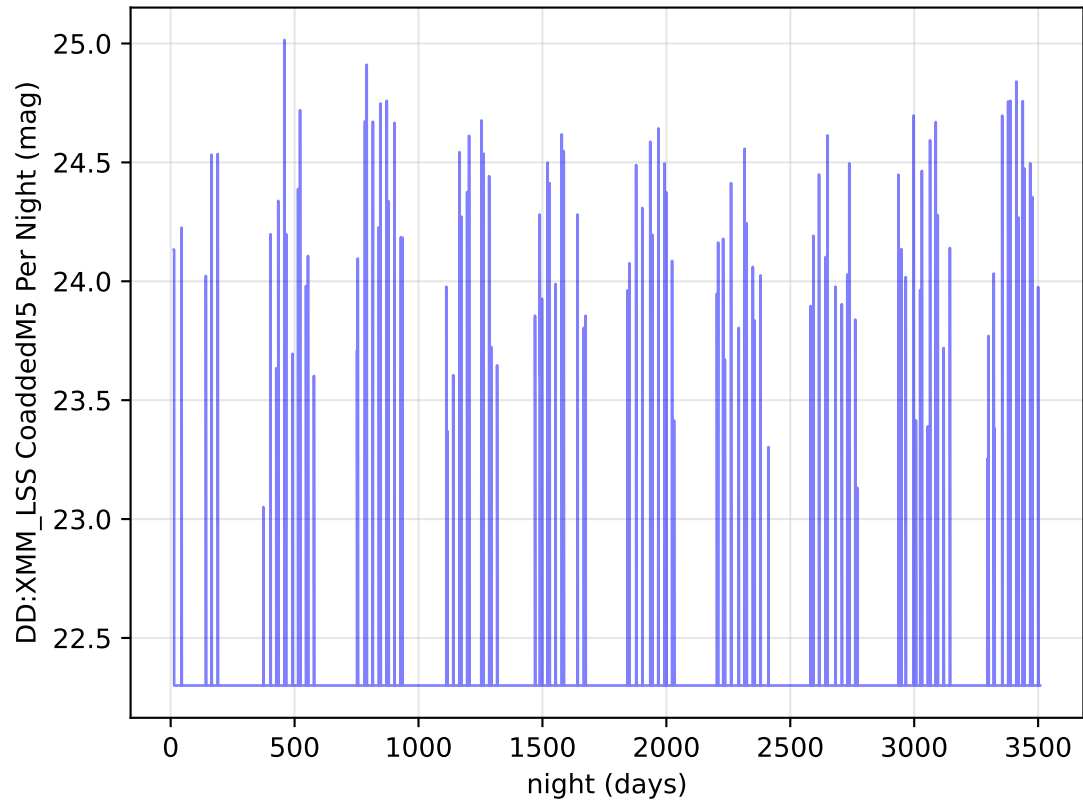
roll_uniform_early_half_mjdp67_v3.4_10yrs u band: DD:XMM_LSS CoaddedM5 Per Night
