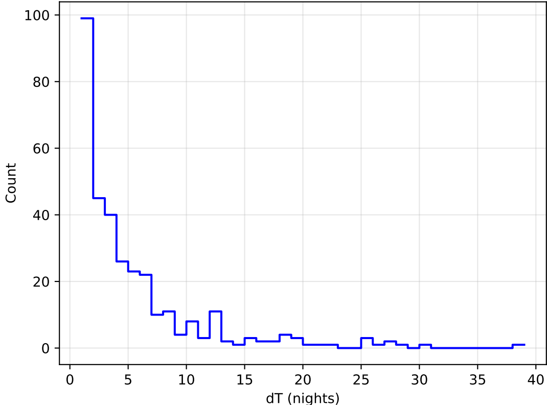
roll_uniform_early_half_mjdp67_v3.4_10yrs all bands: DD:WFD Delta Nights Histogram
