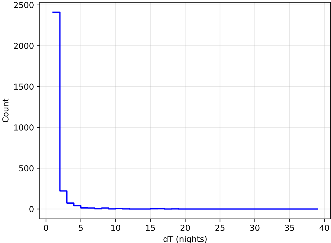
roll_uniform_early_half_mjdp67_v3.4_10yrs all bands: DD:WFD Delta Nights Histogram
