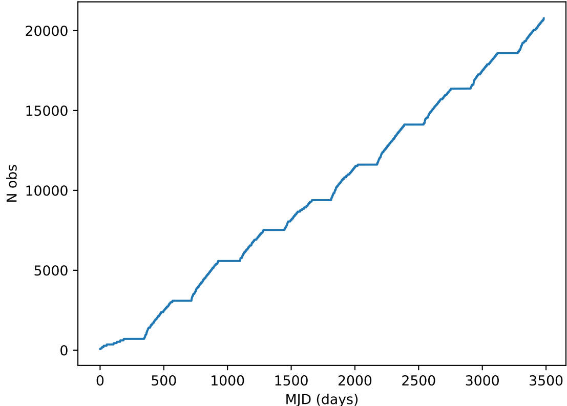
roll_uniform_early_half_mjdp67_v3.4_10yrs all bands: DD:ELAISS1 Cumulative NVisits
