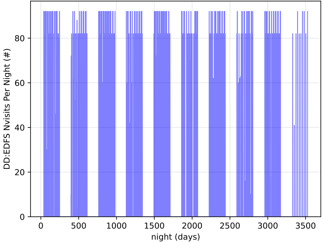
roll_uniform_early_half_mjdp67_v3.4_10yrs all bands: DD:EDFS Nvisits Per Night
