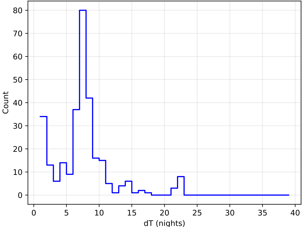
roll_uniform_early_half_mjdp67_v3.4_10yrs all bands: DD:EDFS Delta Nights Histogram
