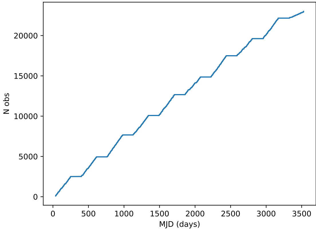
roll_uniform_early_half_mjdp67_v3.4_10yrs all bands: DD:EDFS Cumulative NVisits
