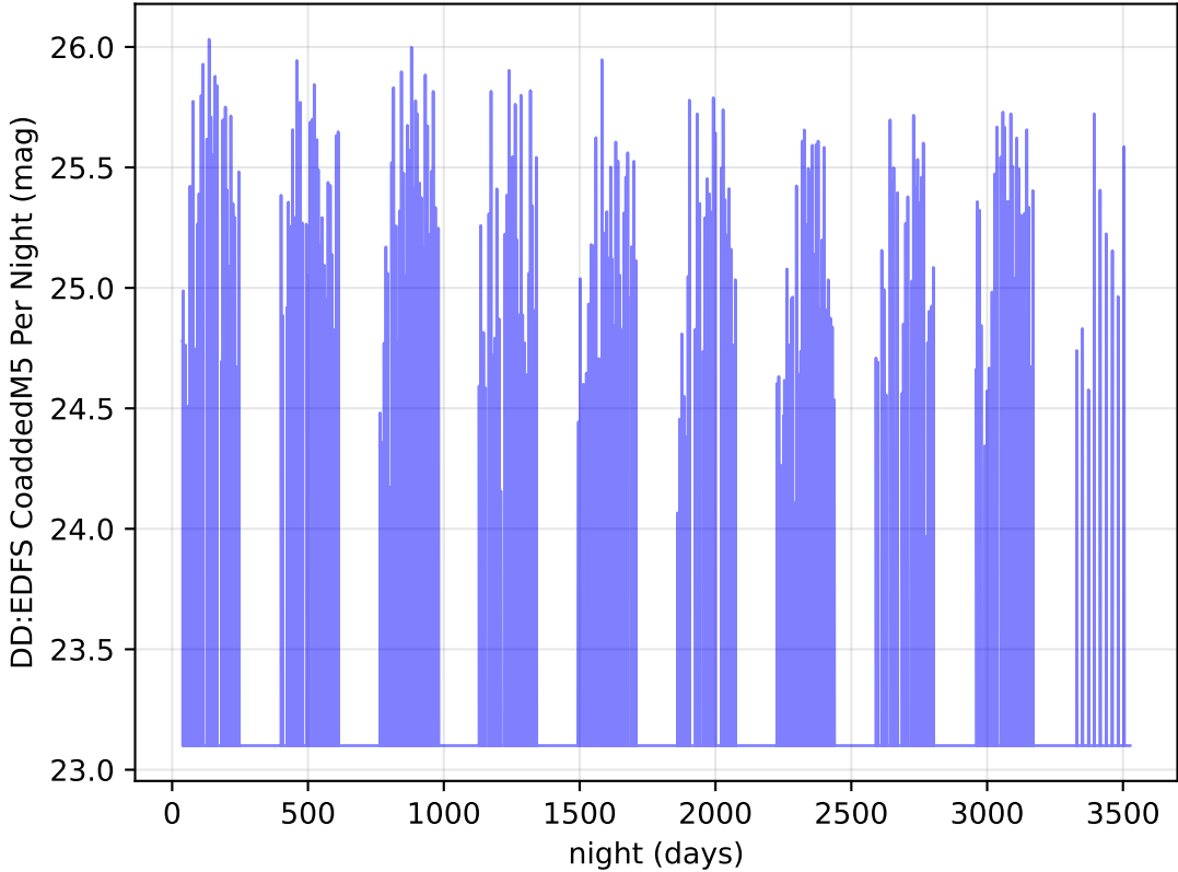
roll_uniform_early_half_mjdp67_v3.4_10yrs i band: DD:EDFS CoaddedM5 Per Night
