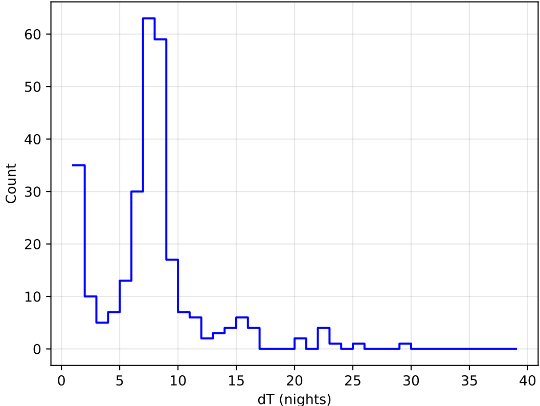
roll_uniform_early_half_mjdp67_v3.4_10yrs all bands: DD:ECDFS Delta Nights Histogram
