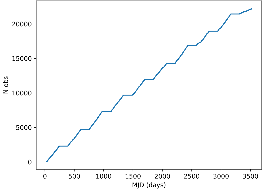
roll_uniform_early_half_mjdp67_v3.4_10yrs all bands: DD:ECDFS Cumulative NVisits
