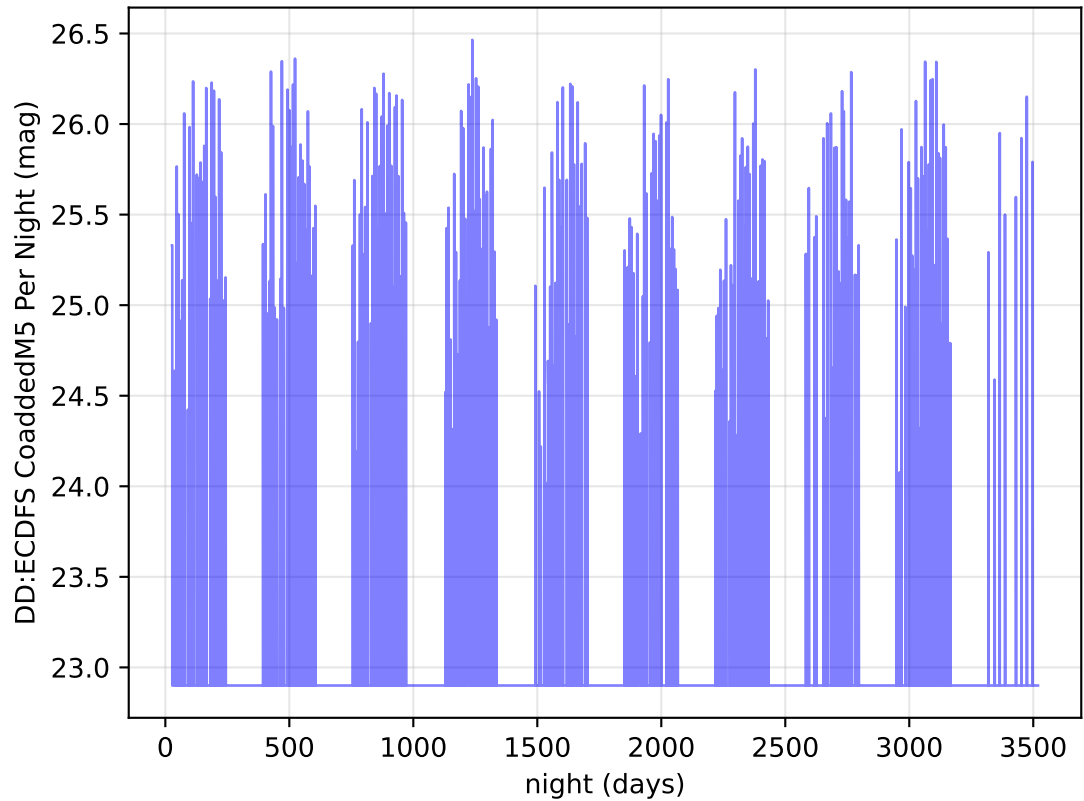
roll_uniform_early_half_mjdp67_v3.4_10yrs r band: DD:ECDFS CoaddedM5 Per Night
