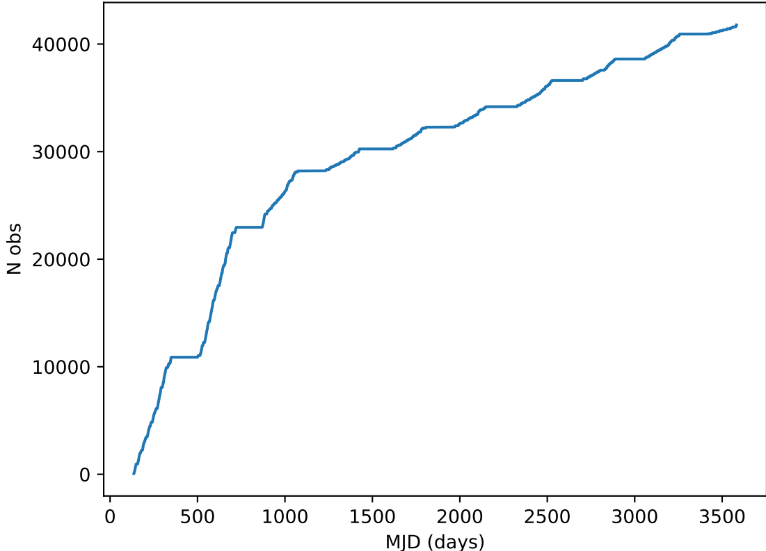
roll_uniform_early_half_mjdp67_v3.4_10yrs all bands: DD: COSMOS Cumulative NVisits
