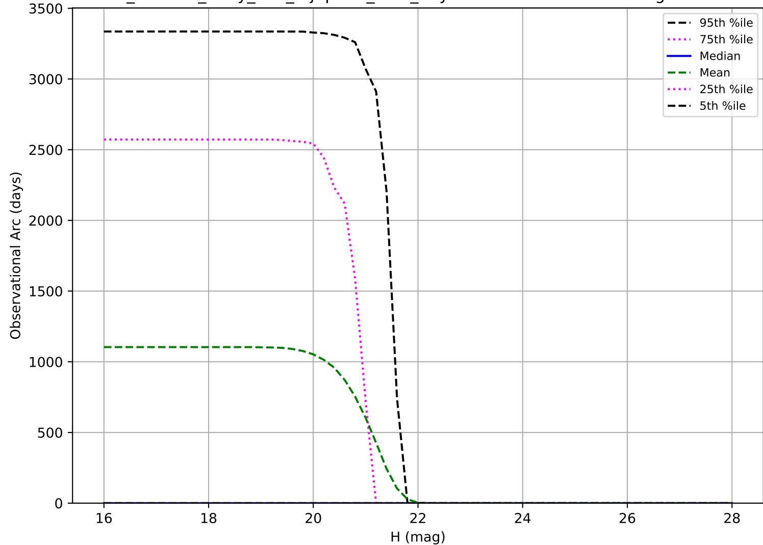
roll_uniform_early_half_mjdp253_v3.4_10yrs: Observational Arc Length Vatira
