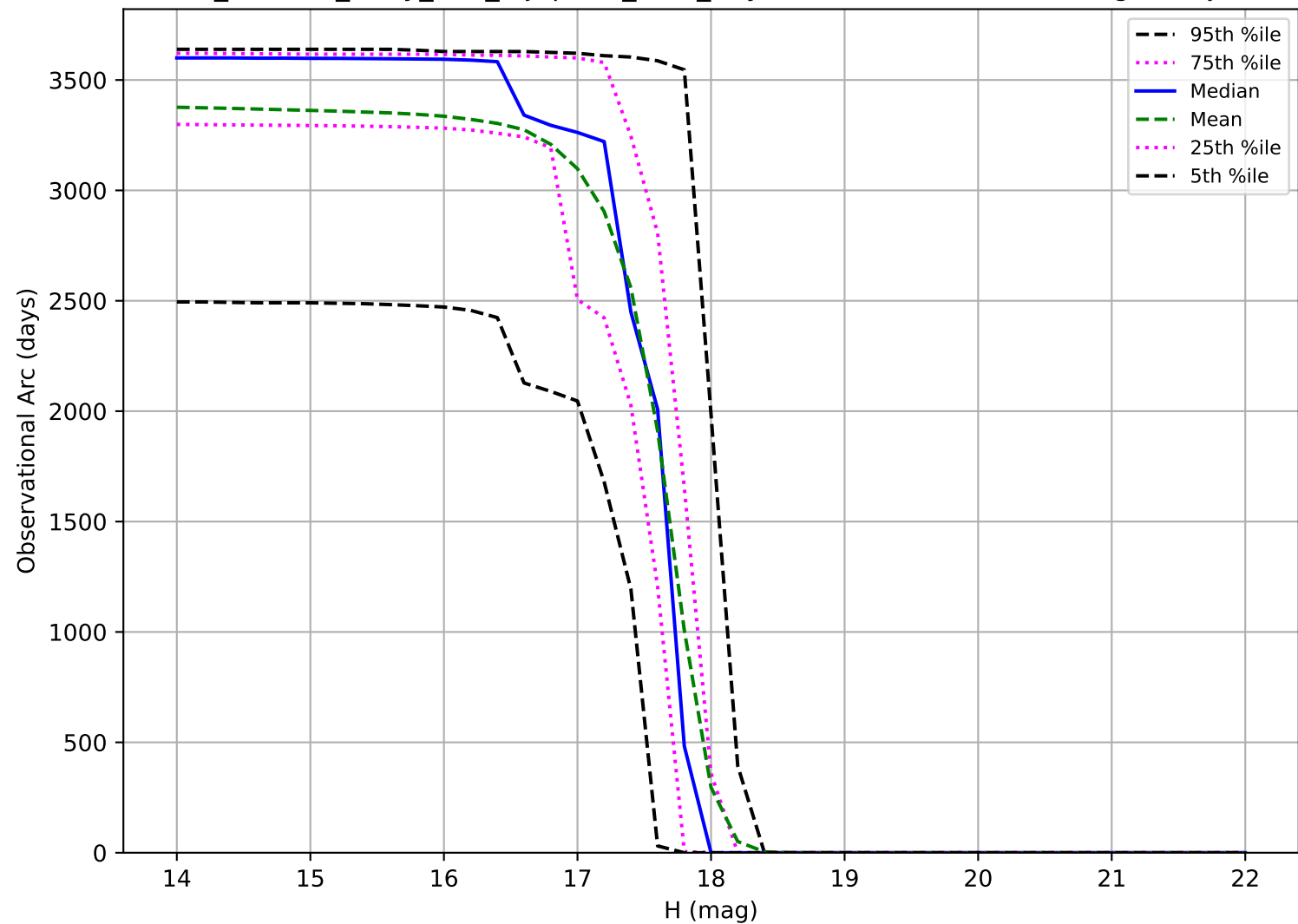
roll_uniform_early_half_mjdp253_v3.4_10yrs: Observational Arc Length Trojan
