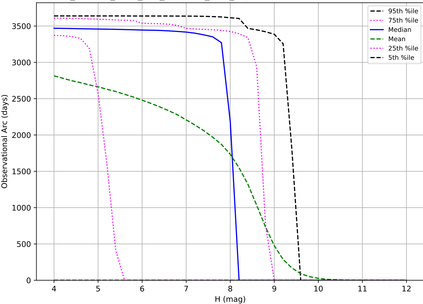
roll_uniform_early_half_mjdp253_v3.4_10yrs: Observational Arc Length TNO
