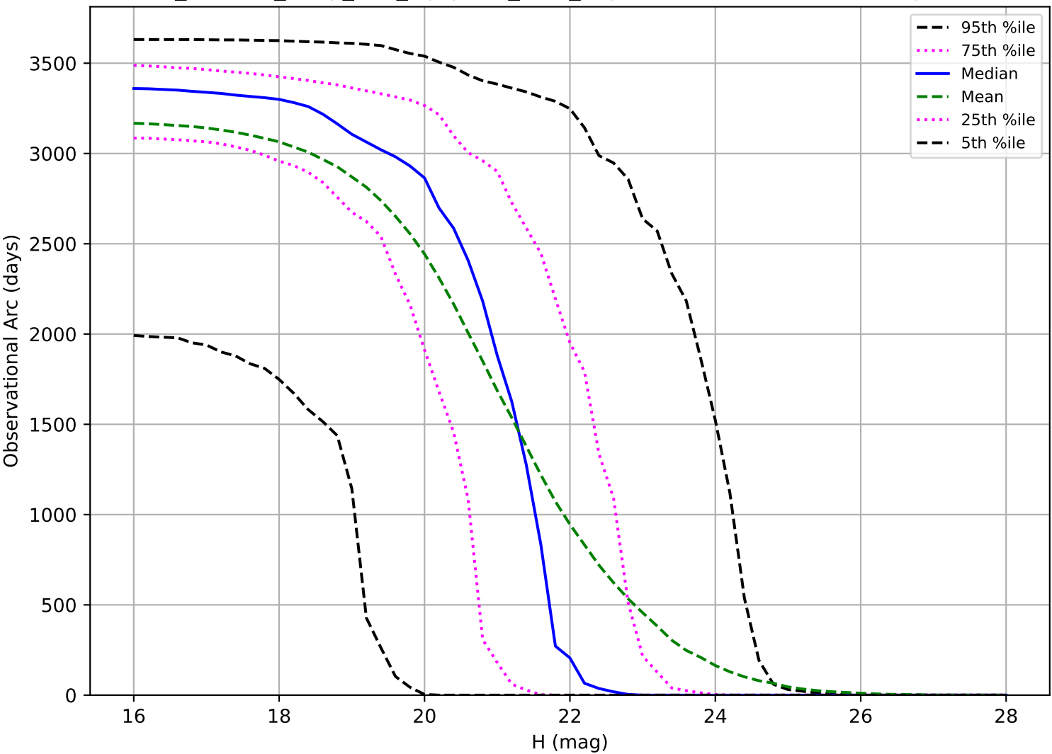
roll_uniform_early_half_mjdp253_v3.4_10yrs: Observational Arc Length PHA
