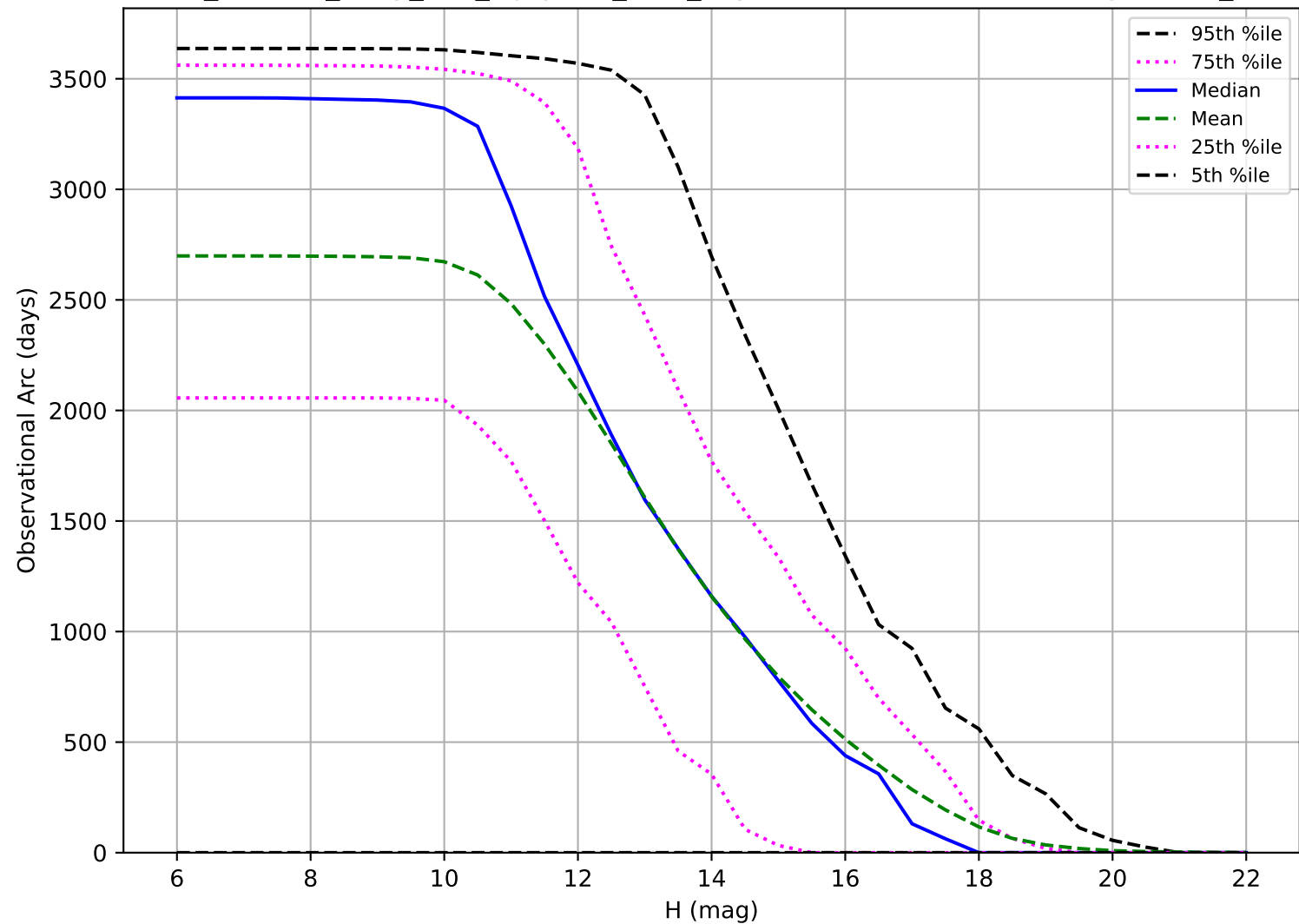
roll_uniform_early_half_mjdp253_v3.4_10yrs: Observational Arc Length OCC_r5
