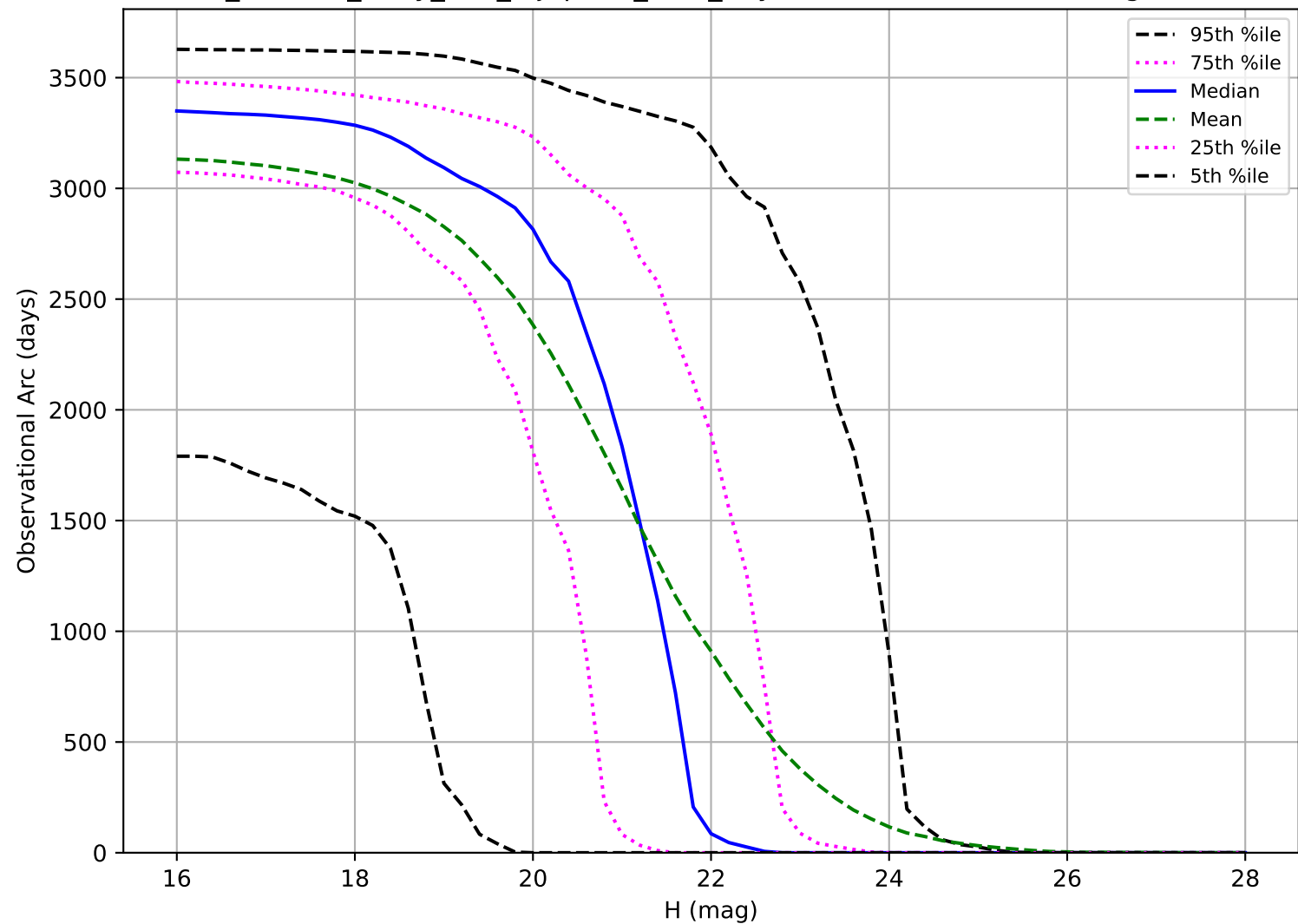
roll_uniform_early_half_mjdp253_v3.4_10yrs: Observational Arc Length NEO
