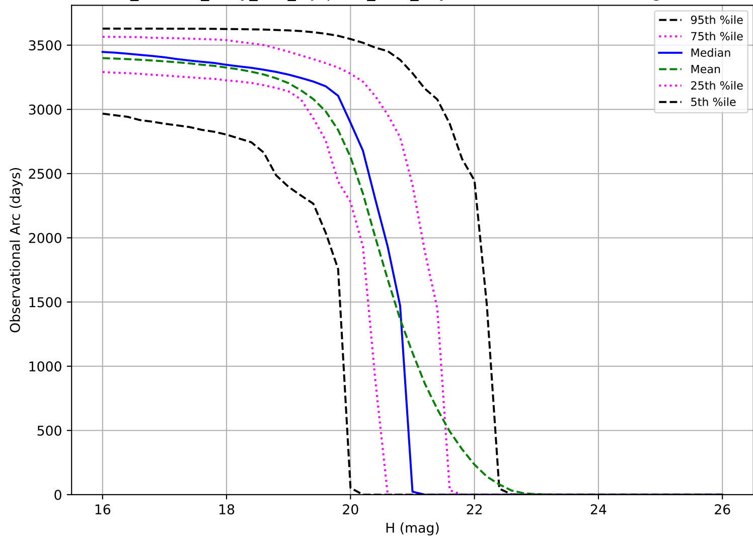
roll_uniform_early_half_mjdp253_v3.4_10yrs: Observational Arc Length MBA
