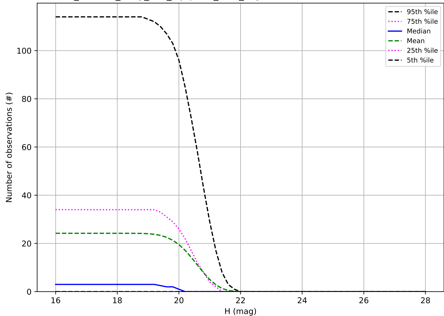
roll_uniform_early_half_mjdp253_v3.4_10yrs: Number of observations Vatira
