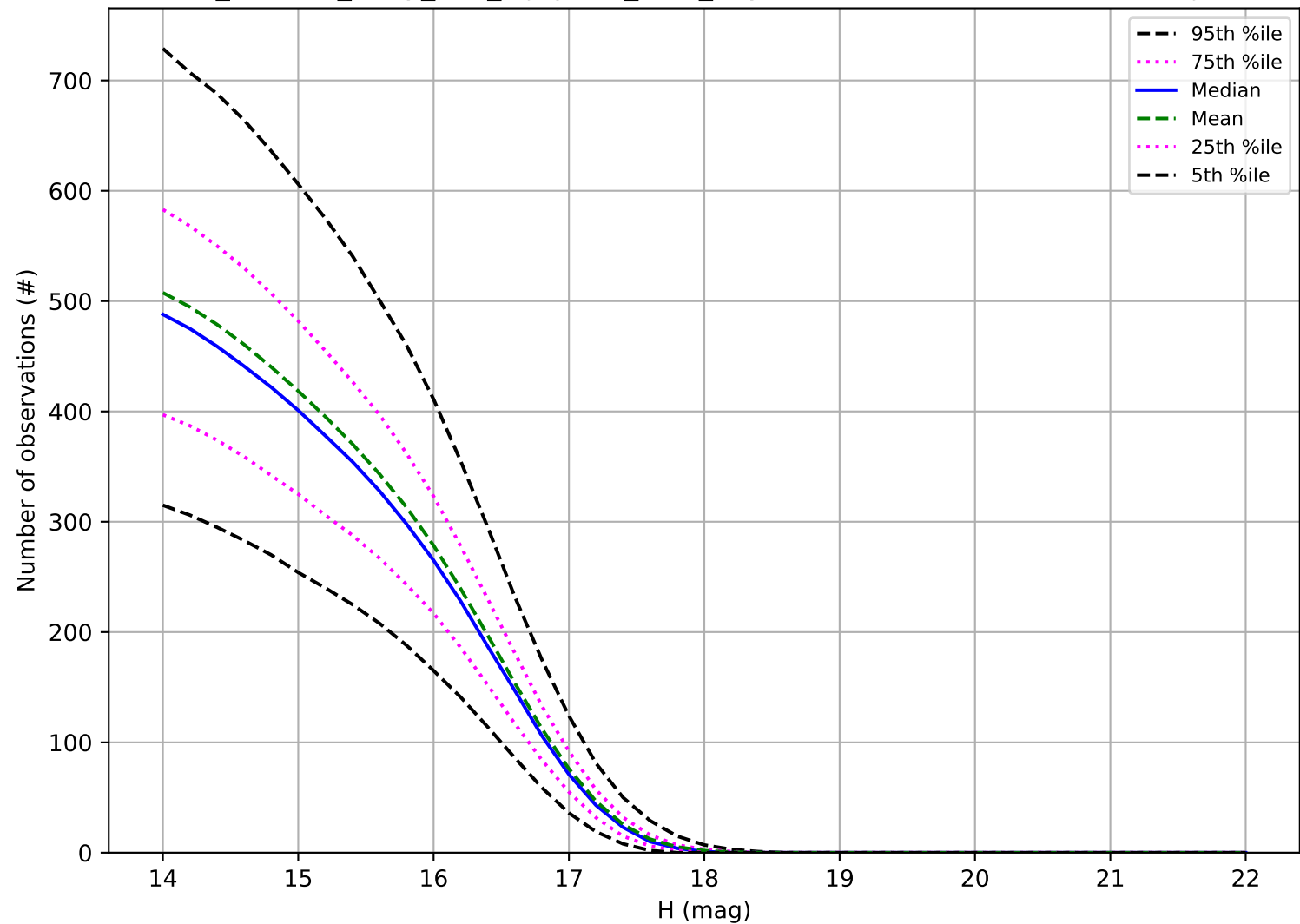
roll_uniform_early_half_mjdp253_v3.4_10yrs: Number of observations Trojan
