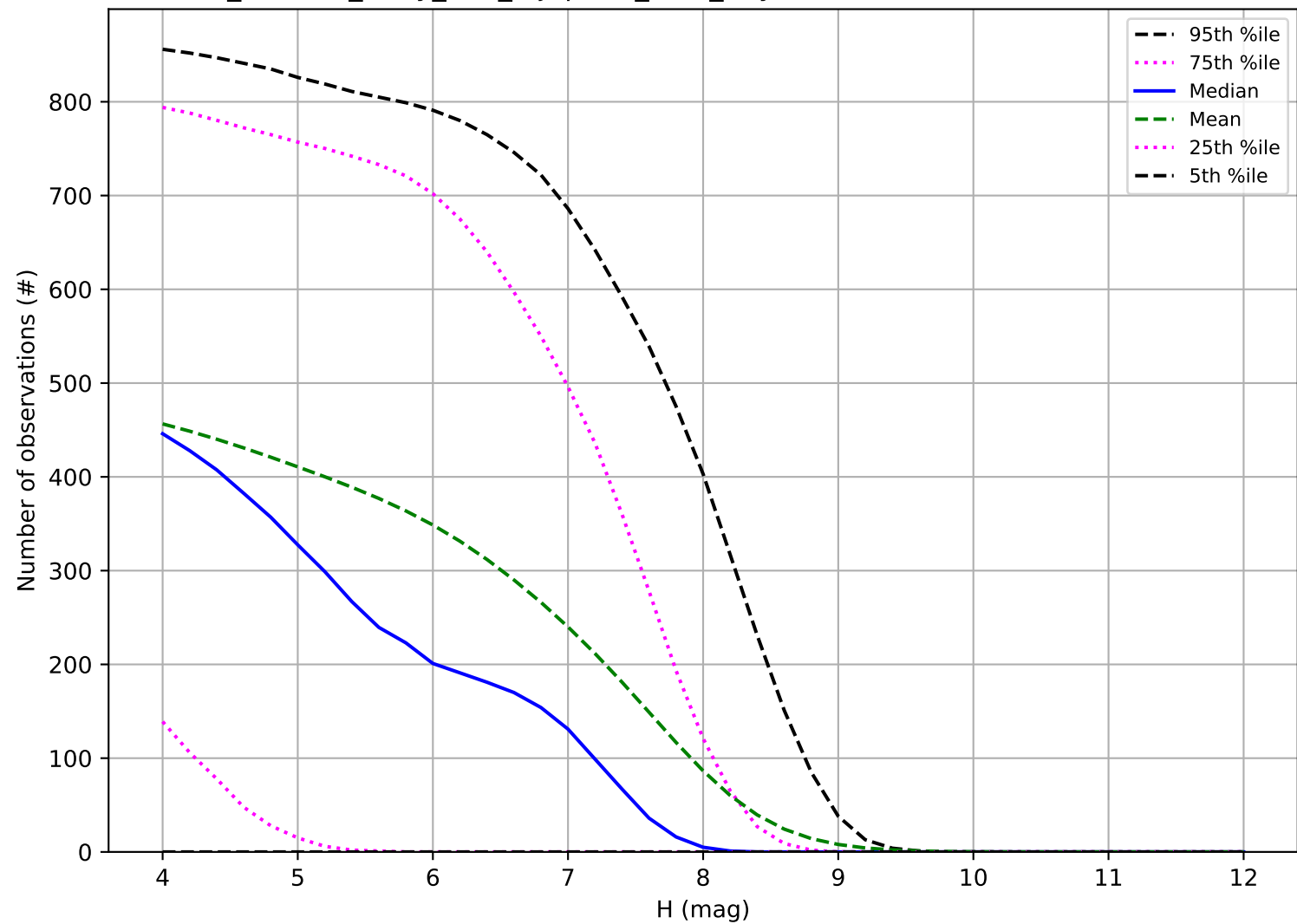
roll_uniform_early_half_mjdp253_v3.4_10yrs: Number of observations TNO
