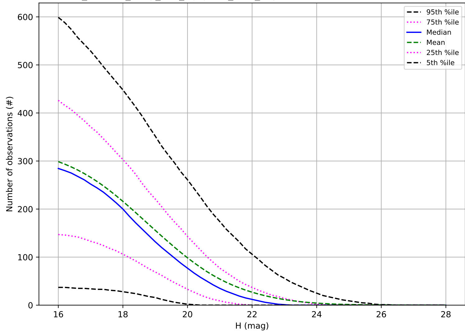
roll_uniform_early_half_mjdp253_v3.4_10yrs: Number of observations PHA
