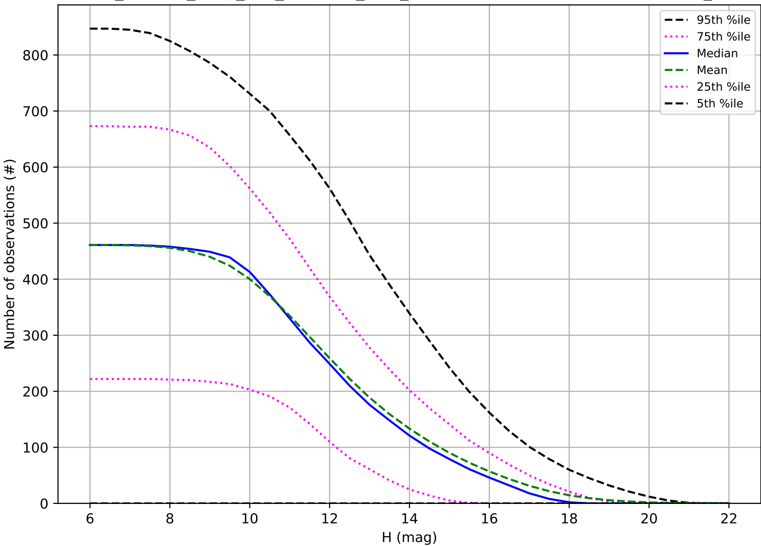
roll_uniform_early_half_mjdp253_v3.4_10yrs: Number of observations OCC_r5
