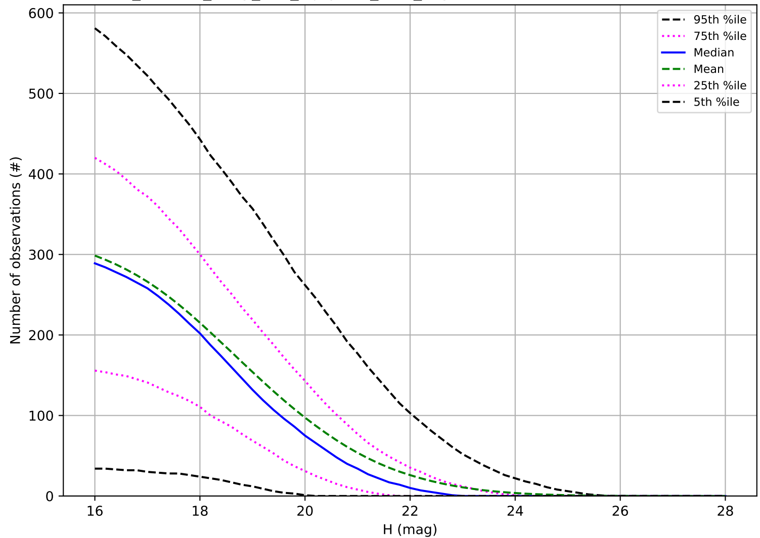
roll_uniform_early_half_mjdp253_v3.4_10yrs: Number of observations NEO
