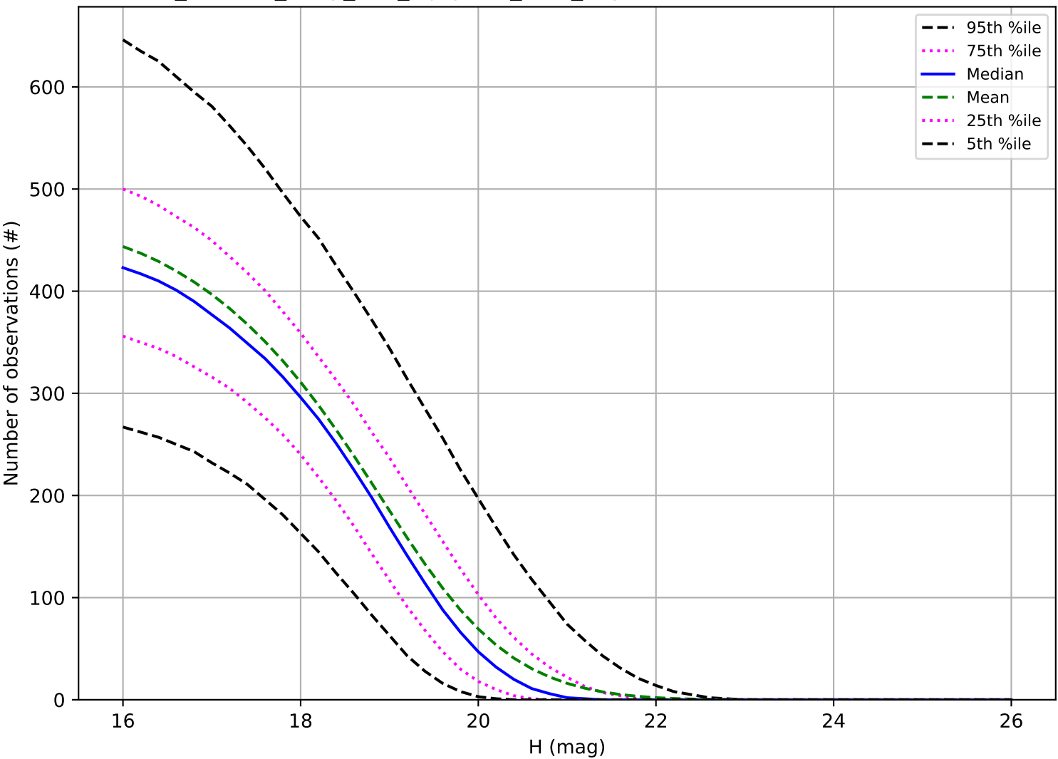
roll_uniform_early_half_mjdp253_v3.4_10yrs: Number of observations MBA
