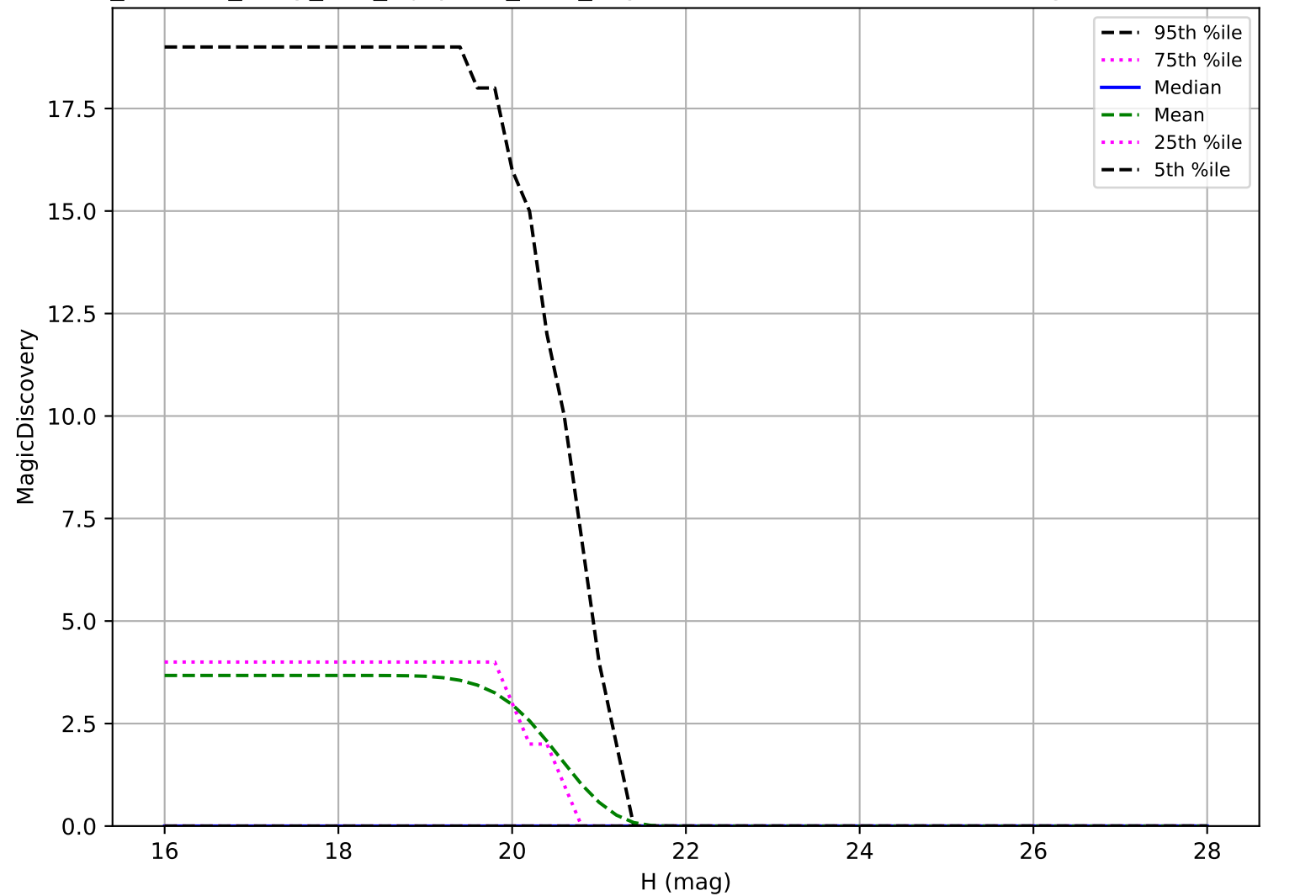
roll_uniform_early_half_mjdp253_v3.4_10yrs: Vatira 6 detections in 60 nights detection loss
