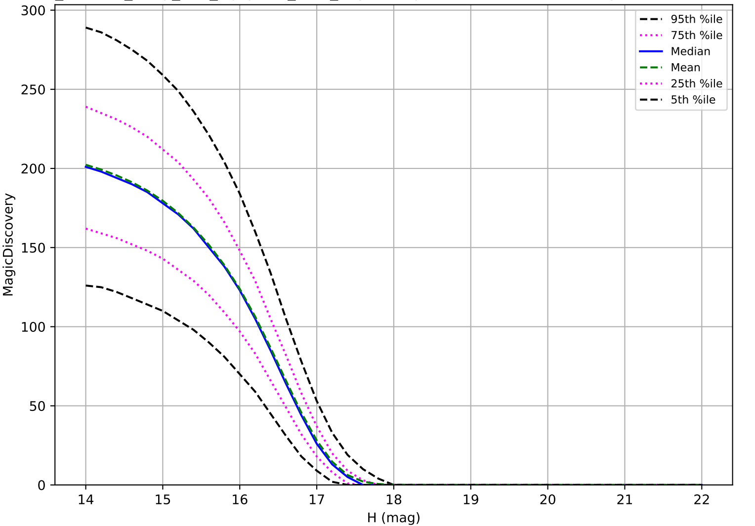
roll_uniform_early_half_mjdp253_v3.4_10yrs: Trojan 6 detections in 60 nights detection loss
