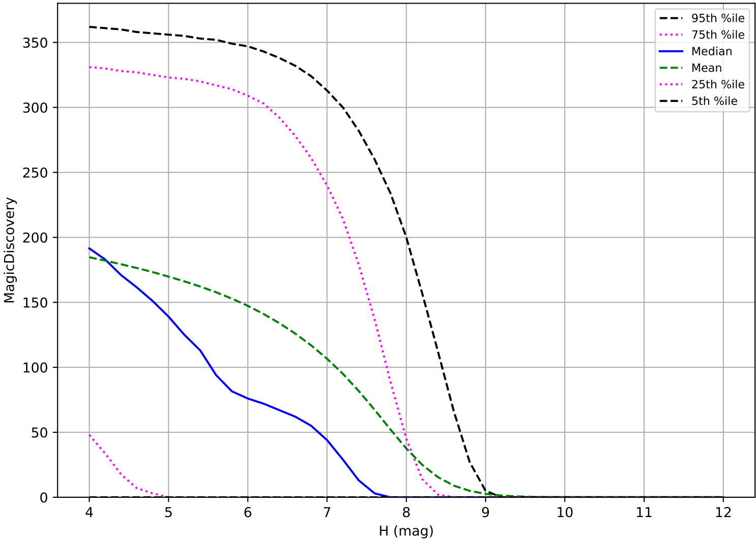
roll_uniform_early_half_mjdp253_v3.4_10yrs: TNO 6 detections in 60 nights detection loss
