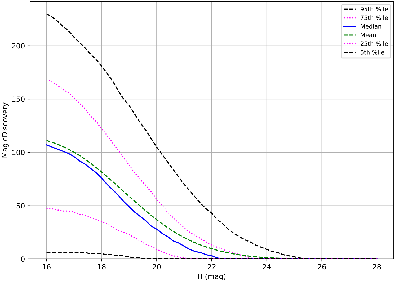
roll_uniform_early_half_mjdp253_v3.4_10yrs: PHA 6 detections in 60 nights detection loss
