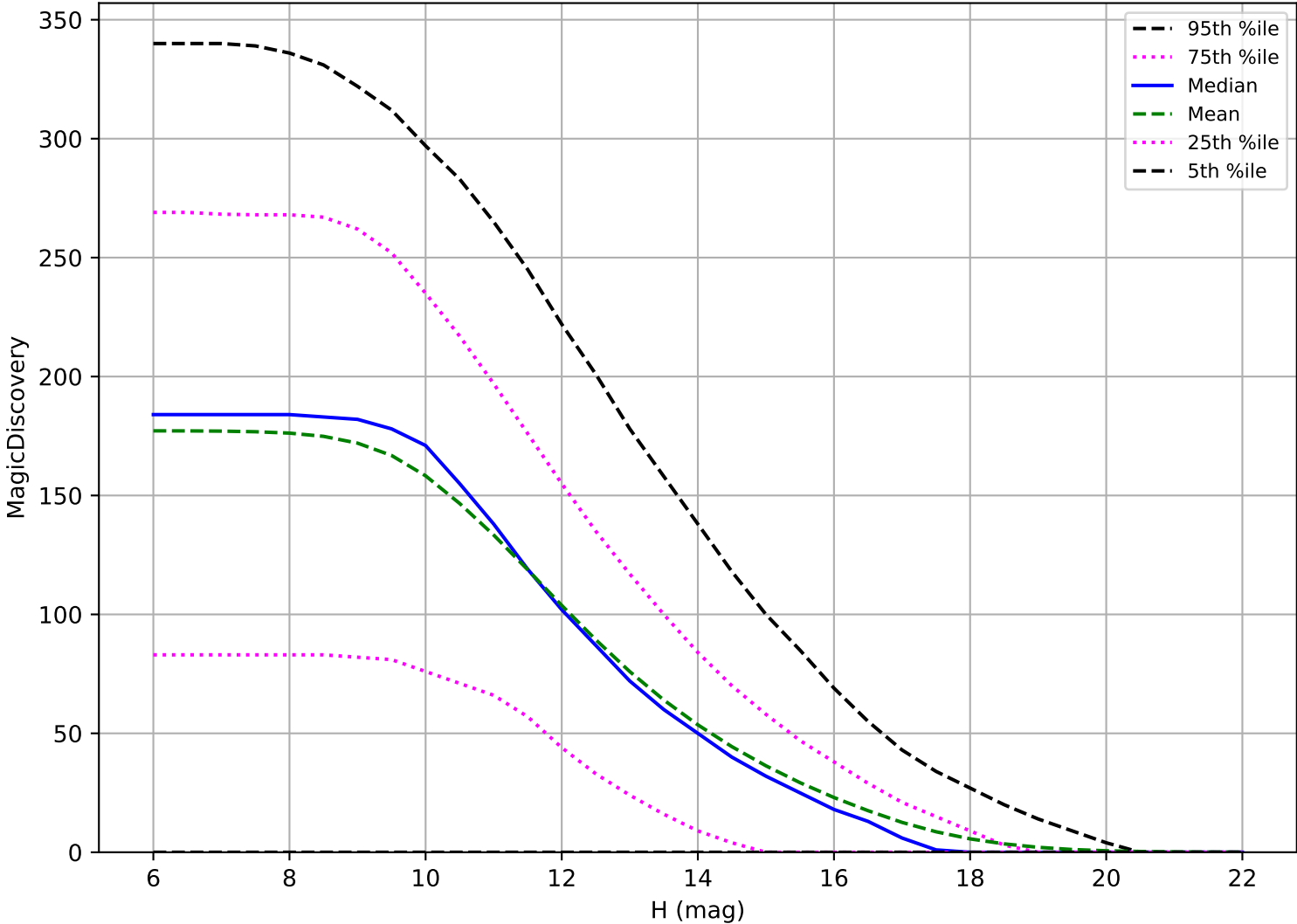
roll_uniform_early_half_mjdp253_v3.4_10yrs: OCC_r5 6 detections in 60 nights detection loss
