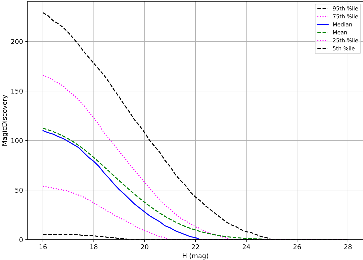
roll_uniform_early_half_mjdp253_v3.4_10yrs: NEO 6 detections in 60 nights detection loss
