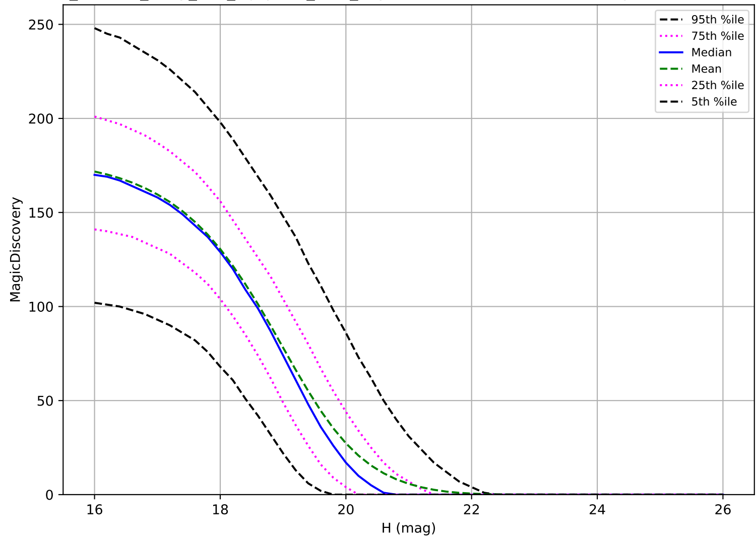
roll_uniform_early_half_mjdp253_v3.4_10yrs: MBA 6 detections in 60 nights detection loss
