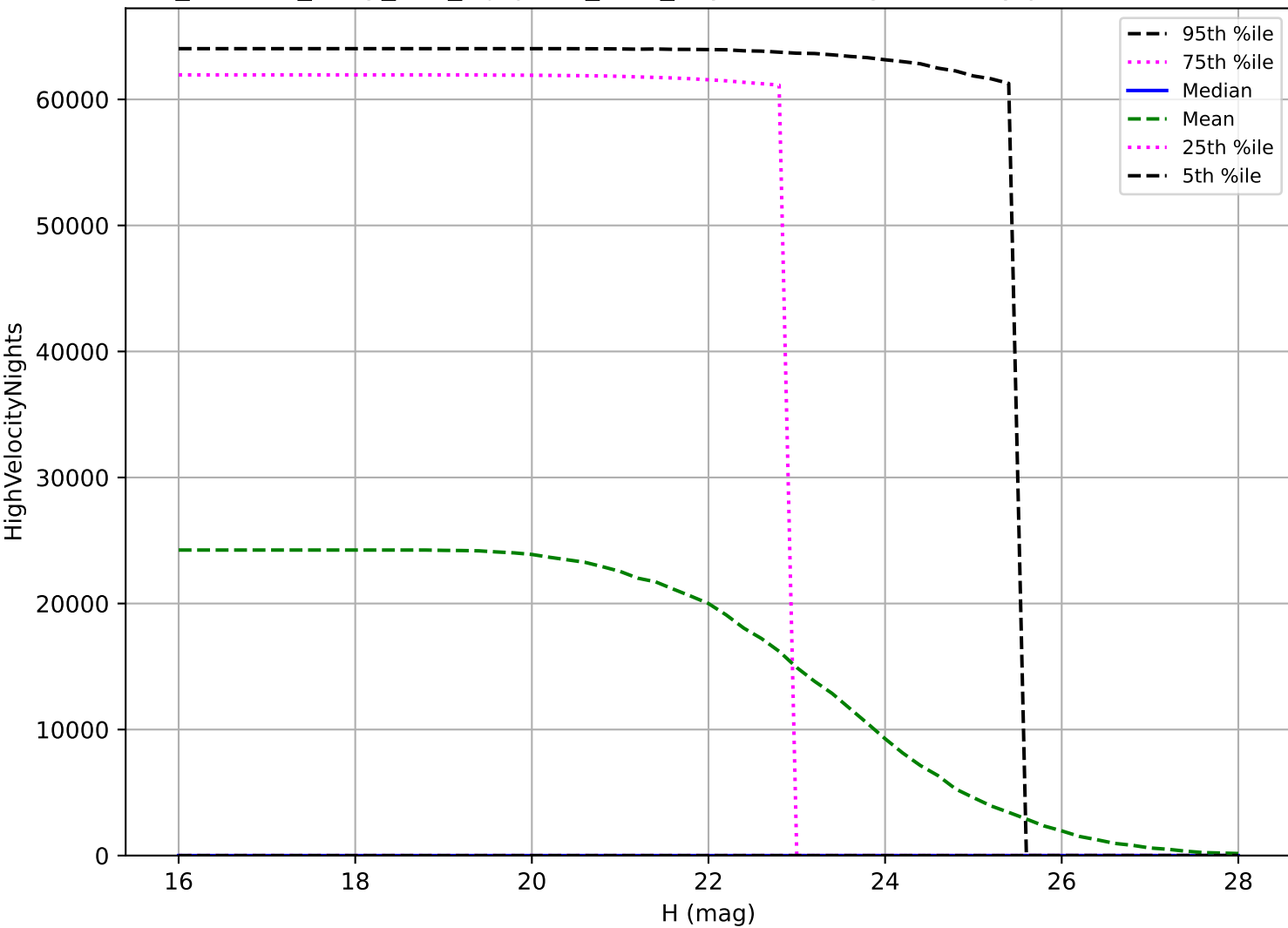
roll_uniform_early_half_mjdp253_v3.4_10yrs: PHA High velocity pair detection loss
