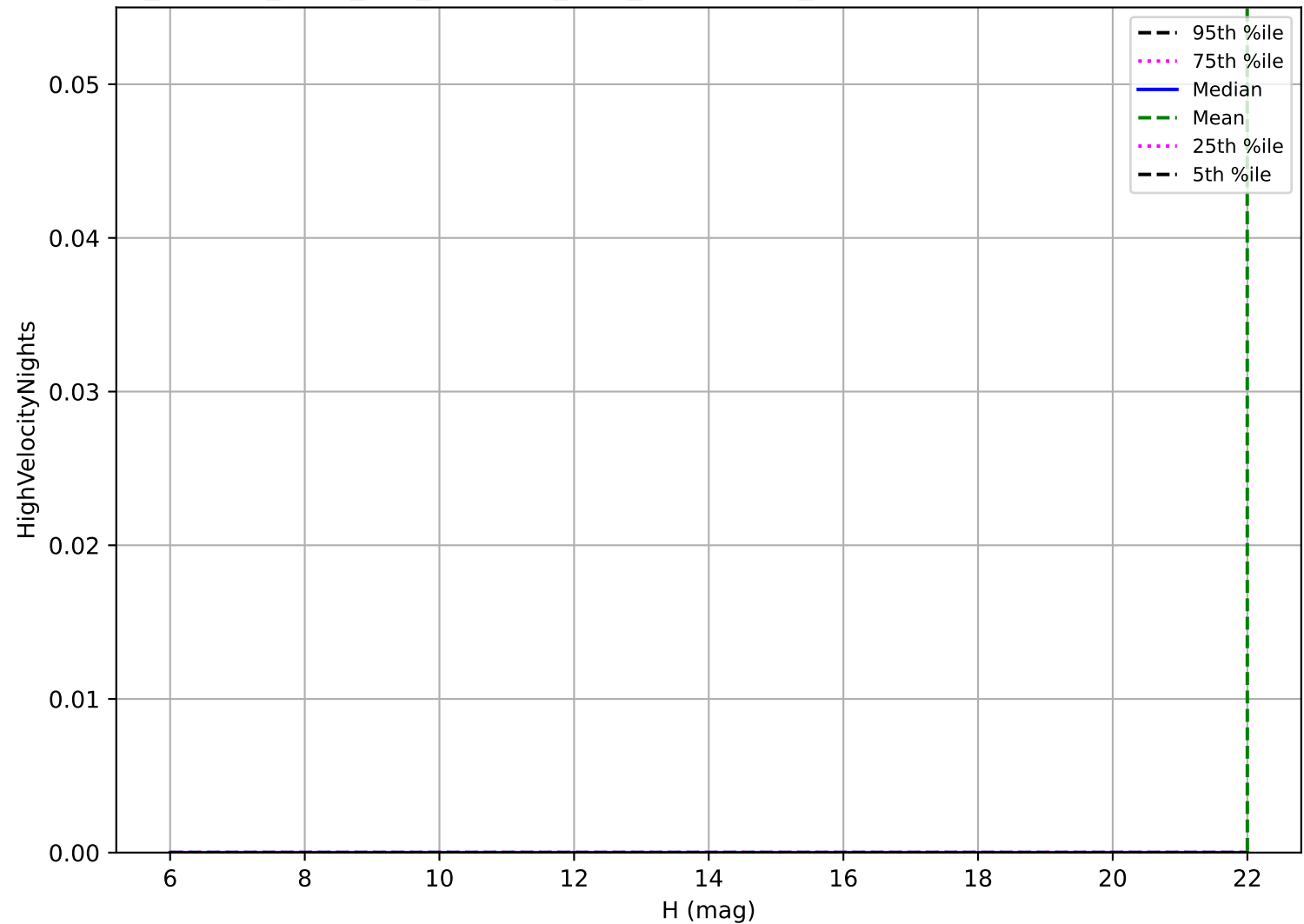
roll_uniform_early_half_mjdp253_v3.4_10yrs: OCC_r20 High velocity pair detection loss
