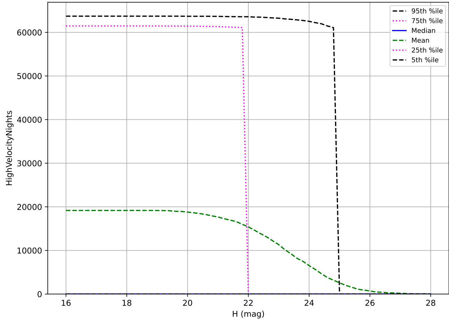
roll_uniform_early_half_mjdp253_v3.4_10yrs: NEO High velocity pair detection loss
