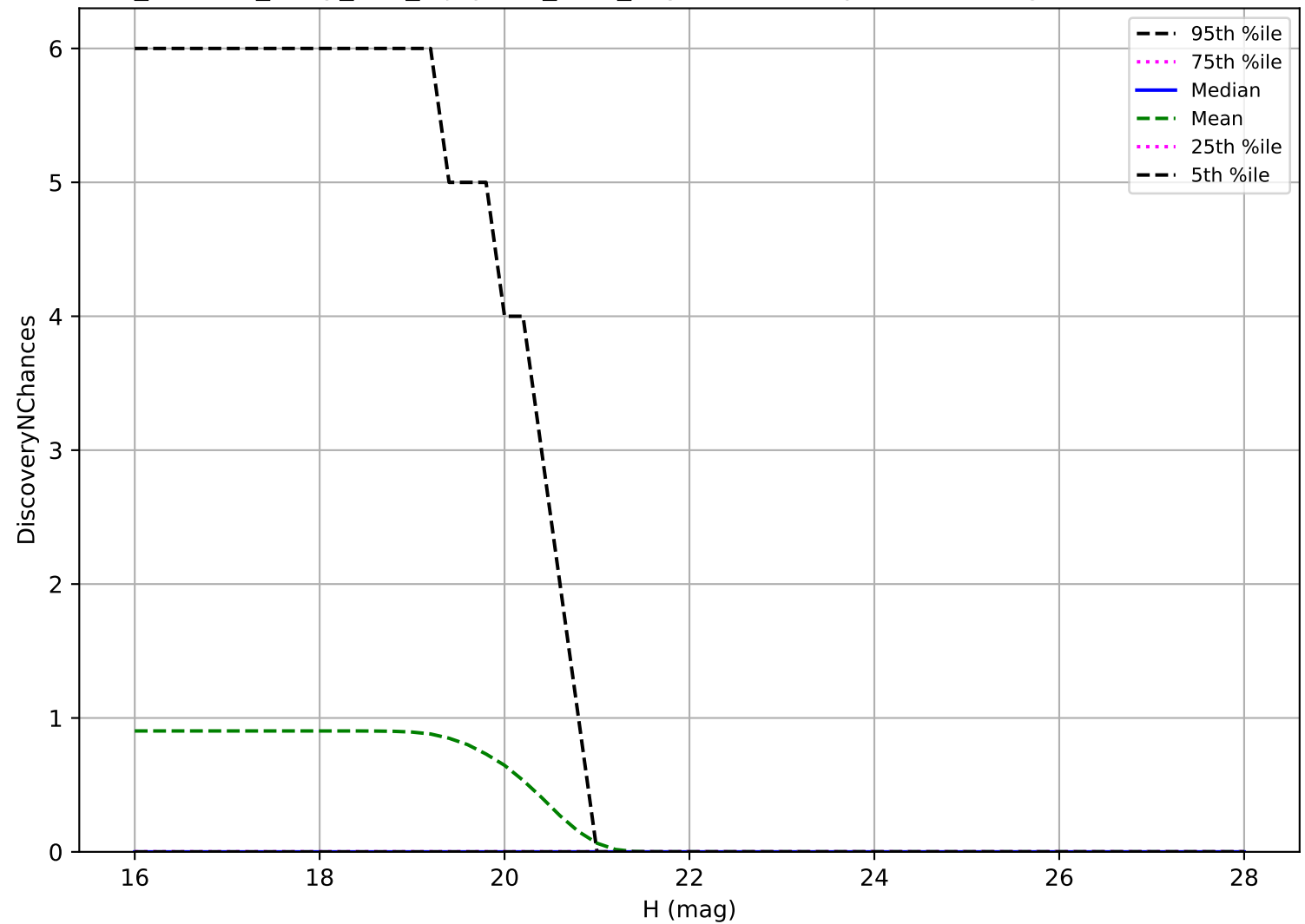
roll_uniform_early_half_mjdp253_v3.4_10yrs: Vatira 3 pairs in 15 nights detection loss
