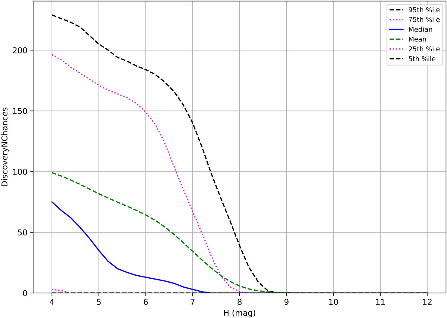
roll_uniform_early_half_mjdp253_v3.4_10yrs: TNO 3 pairs in 15 nights detection loss
