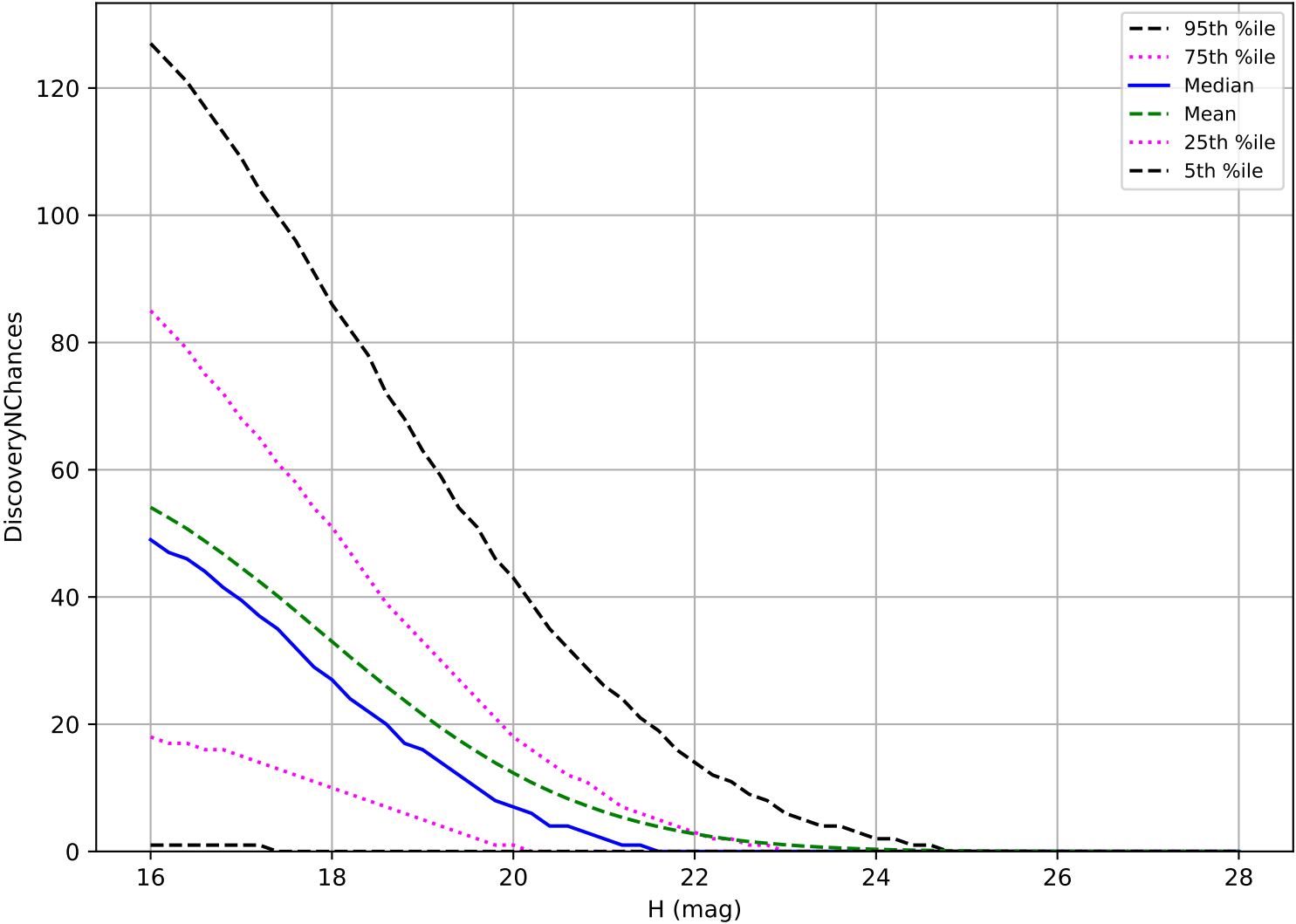
roll_uniform_early_half_mjdp253_v3.4_10yrs: PHA 3 pairs in 15 nights detection loss
