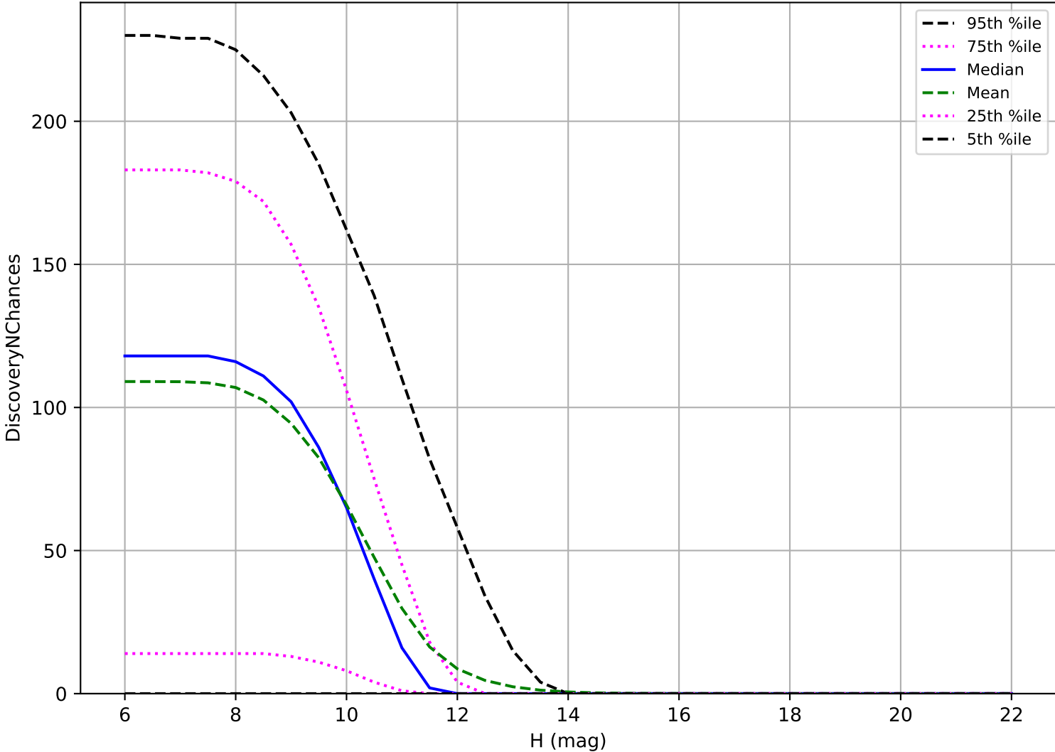
roll_uniform_early_half_mjdp253_v3.4_10yrs: OCC_r20 3 pairs in 15 nights detection loss
