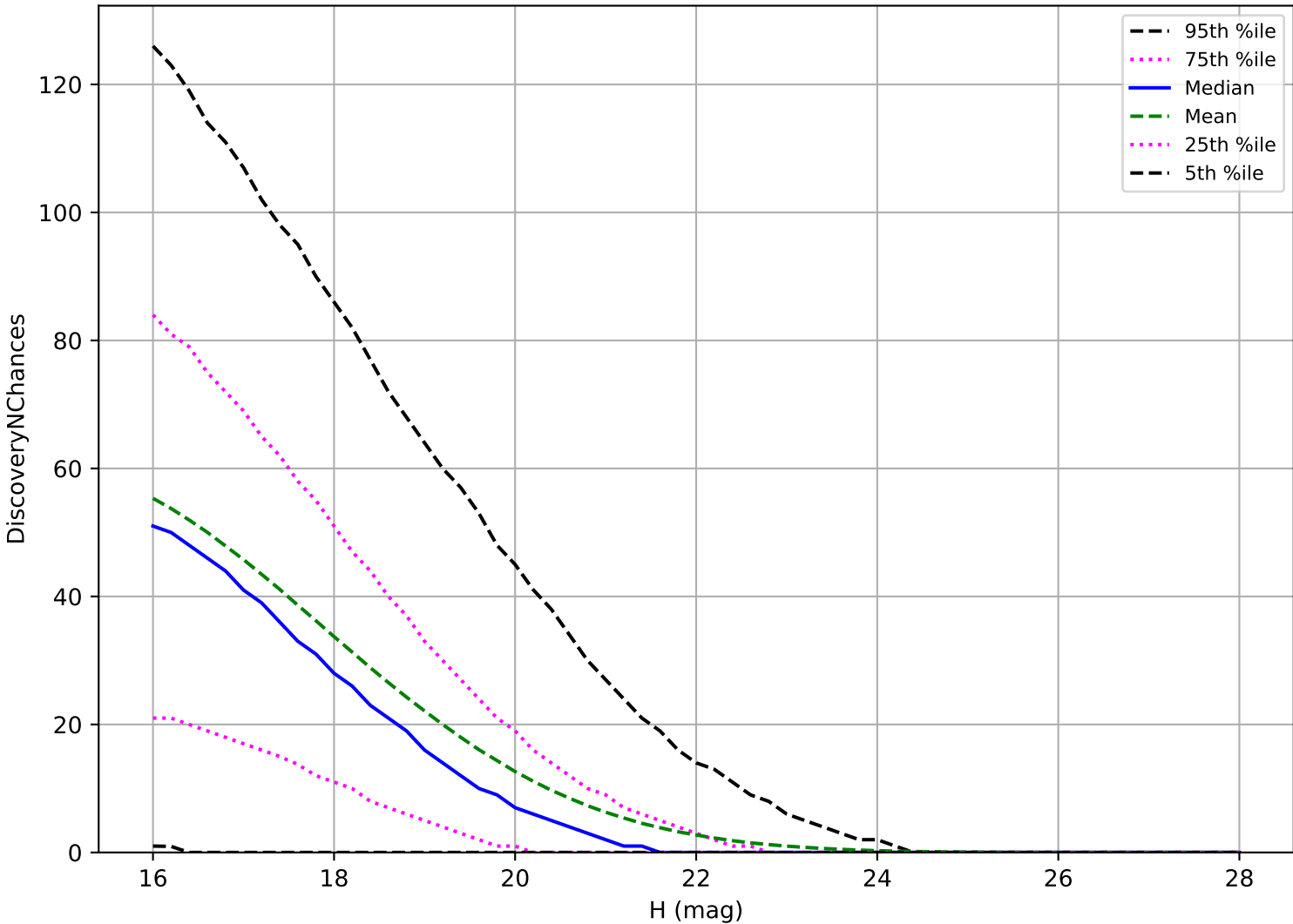
roll_uniform_early_half_mjdp253_v3.4_10yrs: NEO 3 pairs in 15 nights detection loss
